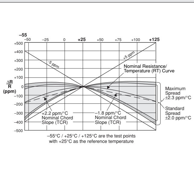
FIGURE 1 - NOMINAL TCR
